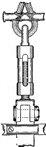
TURNBUCKLE.
